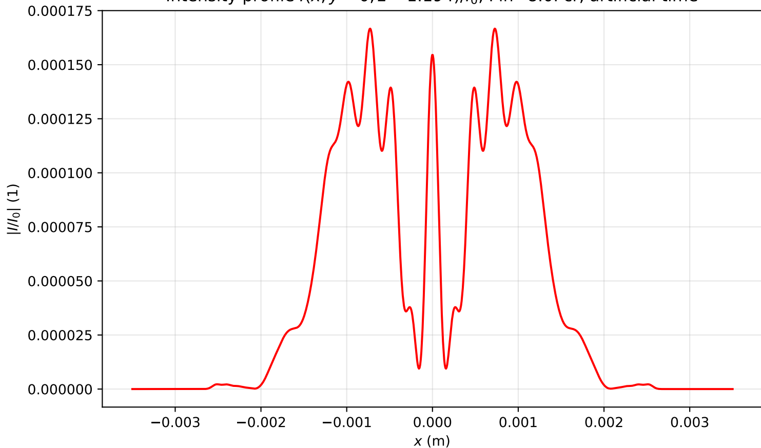
Intensity profile I(x, y = 0, z = 1.194)/I_0 , \text{Pin}=8.0\text{Pcr} , artificial time
